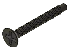
2 X J METAL SCREW PH2 BLACK Ø3.5 L35 mm 630 035 035 PH2 BL
