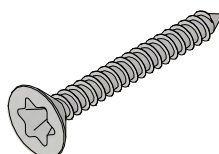
49 X D WOOD SCREW T20 Ø4 L35mm 635 040 035 T20
