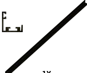
1X BOTTOM RIGHT WINDOW BASE PROFILE L. 570MM 731 HOR B 1123 501
