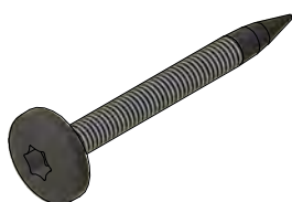
3 X F TRESPA SCREW T20 Ø4.8 L50 mm 637 048 050 T20 511
