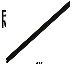
4X HORIZONTAL WINDOW CLICK PROFILE L. 857 MM 731 HOR C 0857 501
