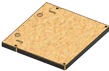
4X FLOORPLATE B 710 P 600 552 201
