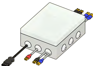
DIMMABLE JUNCTION BOX 3 VENTILIGHT 791 001 051 3V
